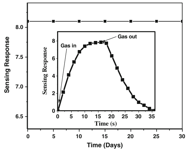
Fig. 11 Stability characteristics of 80 wt% graphene/ Al_2O_3 chemiresistor to 100 ppm CO_2 . Inset shows Transient response of 80 wt% graphene/ Al_2O_3 chemiresistor to 100 ppm CO_2
