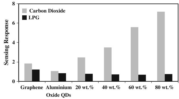
Fig. 7 Comparative gas sensing responses of chemiresistors towards CO 2 and LPG for 40 ppm at 398 K
